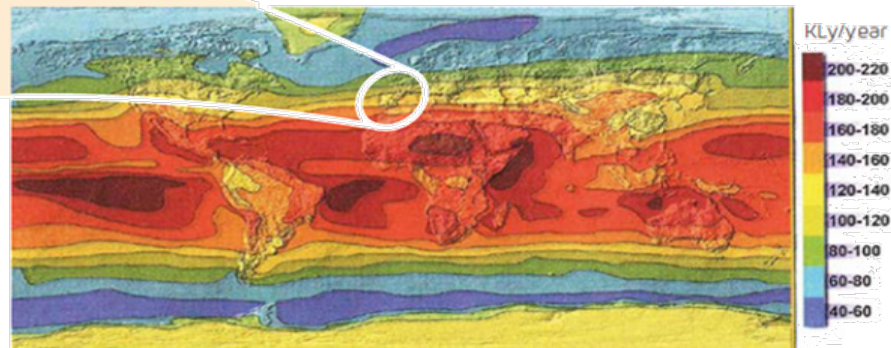
Worldwide distribution of global solar radiation
